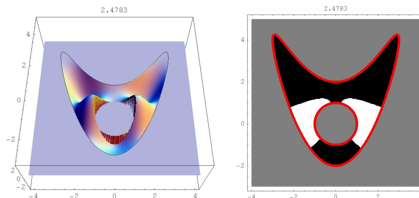
Figure 3: Eigenmode for the 6th eigenfrequency: plot and nodal domains.
