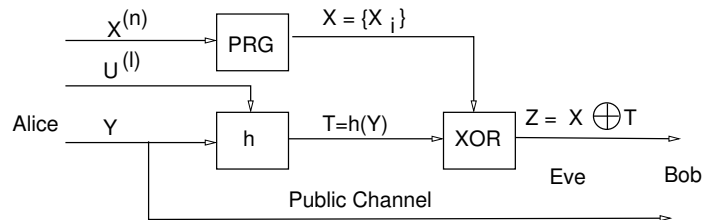
Figure 1: Brassard's classical authentication protocol [7]
