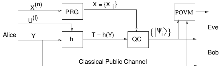
Figure 2: First proposal of quantum-enhanced authentication scheme
