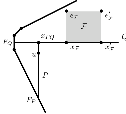
FIGURE 3.1.1. An extended probe with flag \mathcal{FP} = P \cup Q \cup \mathcal{F} .
