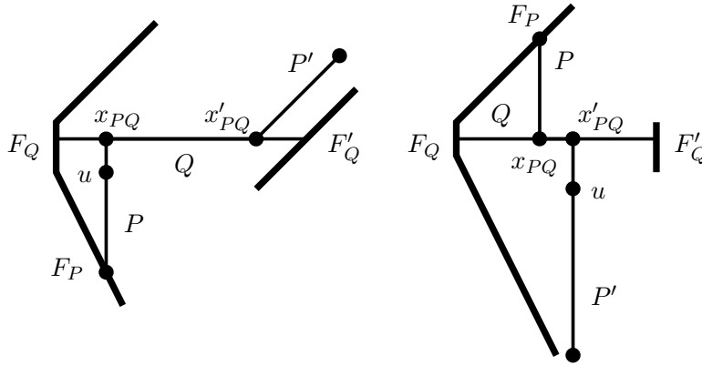
FIGURE 2.2.1. Two ways of using Theorem 2.2.6. Left: u is on P . Right: u is on P' .
