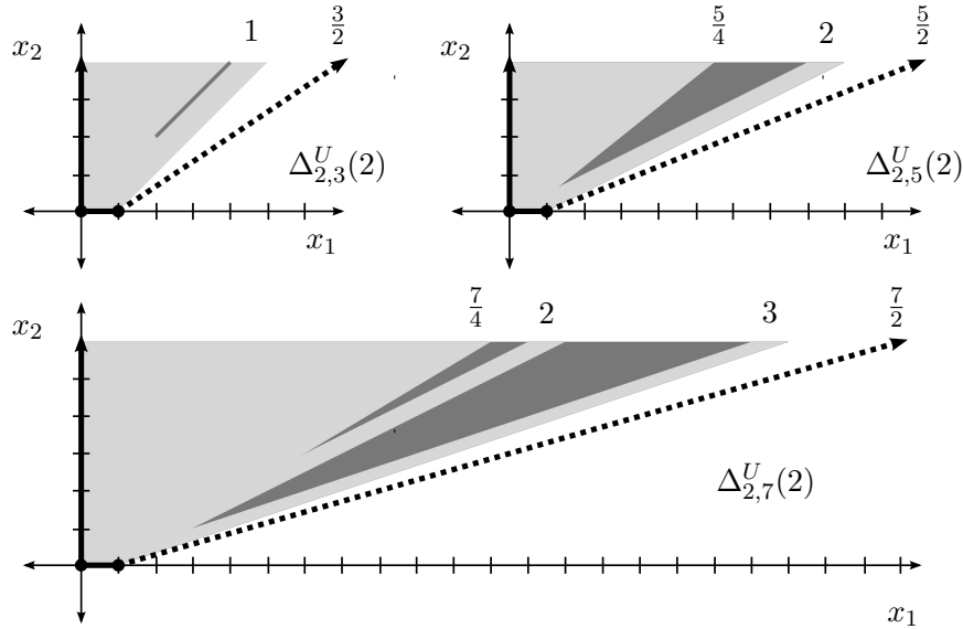
FIGURE 3.2.2. Comparing Lemma 3.2.1 and Lemma 3.2.2. The points in the gray regions are displaceable, but extended probes are needed for points in the dark gray regions. See Remark 3.2.3. In this figure and others the numbers 1, \frac{3}{2}, \frac{5}{4}, 2, \dots refer to the slope \lambda for the line x_1 = \lambda x_2 + b defining the boundary between differently shaded regions.
