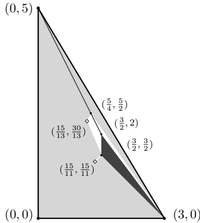
FIGURE 4.6.1. The moment polytope for \mathbb{P}(1, 3, 5) . The probe displaceable points in light gray, the nondisplaceable points in dark grey, and the unknown points in white.
