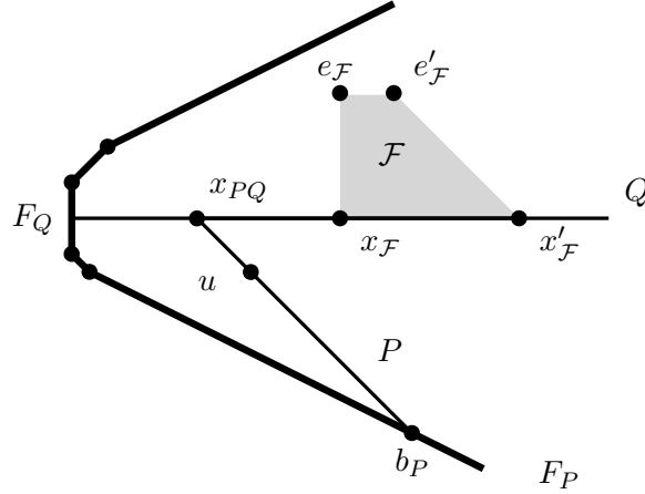
FIGURE 5.2.1. An extended probe with flag \mathcal{FP} = P \cup Q \cup \mathcal{F}_{\mu} , where the flag parameter \mu = 0 .
