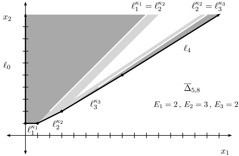
FIGURE 4.5.3. Displaceable fibers in \overline{\Delta}_{5,8}(\kappa) . The light grey regions are displaceable by standard probes with direction (1, 1) , (3, 2) , or parallel to one of the added facets. The medium gray regions are displaceable by extended probes from Proposition 4.4.4. Displaceability is unknown for points in the white rays and regions.
