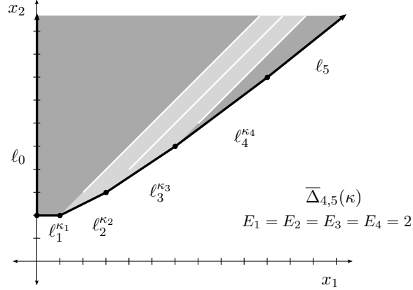
FIGURE 4.5.2. Minimal resolution of A_n -singularity. The light grey regions are displaceable by standard probes with direction (1,1) or parallel to one of the added facets. The medium grey regions are displaceable by extended probes from Proposition 4.4.4. Displaceability for the white rays is unknown.
