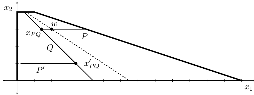
FIGURE 2.3.2. The symmetric extended probe \mathcal{SP} that displaces w when 1 < w_2 < 2 .
