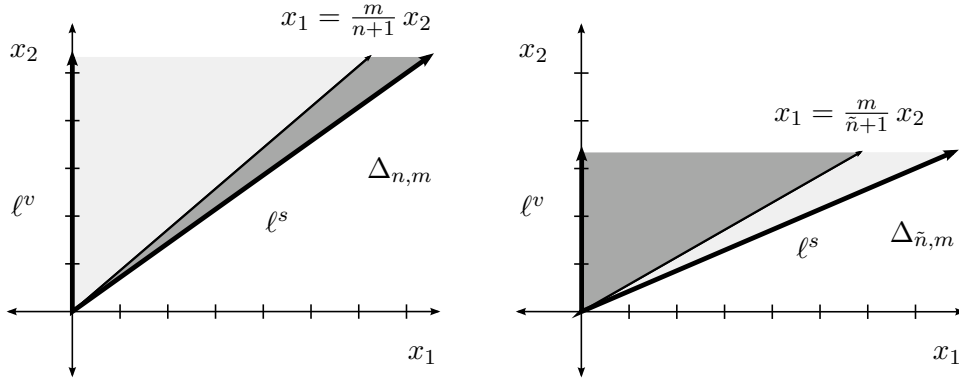
FIGURE 4.3.2. Left: \Delta_{n,m} . Right: \Delta_{\tilde{n},m} . The matrix S in (4.3.6) maps \Delta_{\tilde{n},m} to \Delta_{n,m} , mapping the light gray region to the light gray region, and likewise for the dark gray regions. Here (n, m) = (5, 7) and (\tilde{n}, q) = (3, 2) .
