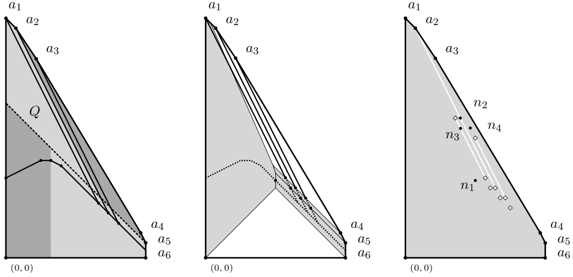
FIGURE 4.6.3. Displaceable and nondisplaceable fibers when both singularities in \mathbb{P}(1, 3, 5) are resolved as in (4.6.10). Left: In grey, points displaceable by symmetric extended probes that use Q , which is based on \{\ell_6^{\kappa_6} = 0\} , as the deflecting probe. Middle: Displacing some more points with standard probes that have direction \pm(1, -1) . Right: In light grey are the fibers that were displaced in the previous two pictures. The white line segments are on the lines from (4.6.11). The point n_1 is nondisplaceable just as in Proposition 4.6.1. The point n_3 satisfies \ell_1 = \ell_4^{\kappa_4} = \ell_6^{\kappa_6} , the point n_2 satisfies \ell_4^{\kappa_4} = \ell_5^{\kappa_5} = \ell_6^{\kappa_6} , the point n_4 satisfies \ell_5^{\kappa_5} = \ell_3 = \ell_6^{\kappa_6} , and all three points are nondisplaceable. Displaceability is unknown for points on the white line segments and the points marked with white diamonds. See Remark 4.6.3.
