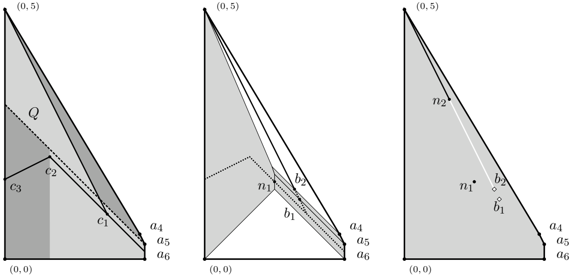
FIGURE 4.6.2. Displaceable and nondisplaceable fibers when the singularity at (3, 0) in \mathbb{P}(1, 3, 5) is resolved as in (4.6.4). Left: In grey, points displaceable by symmetric extended probes deflected by a probe Q , that is based on the edge F_6 with conormal (-2, -1) . Middle: Displacing some more points with standard probes that have direction \pm(1, -1) . Right: In light grey are the fibers that were displaced in the previous two pictures. The point n_1 and the points on the black line segment connecting (0, 5) and n_2 are nondisplaceable. Displaceability is unknown for points on the white line segment, and the points b_1 , and b_2 .
