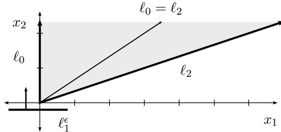
FIGURE 4.2.1. The moment polytope \Delta_{1,m} when m = 3 . The displaceable points are in light gray and the nondisplaceable points are on the line \ell_0 = \ell_2 . The nondisplaceability proof uses ghost facets \{\ell_1^\epsilon(x) \geq 0\} for varying \epsilon \geq 0 .
