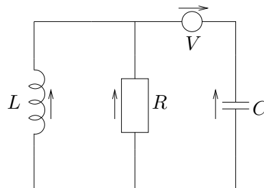
Figure 1.9.: RCL network
