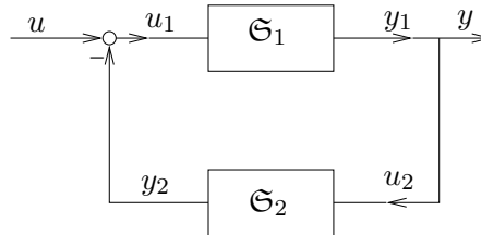
Figure 12.4.: Feedback connection
