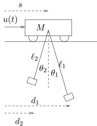
Figure 3.3.: Cart with two pendulums
