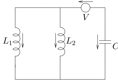
Figure 3.2.: Electrical network
