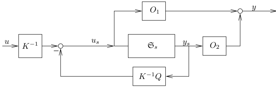
Figure 14.2.: The system (14.11) with input (14.14) and output (14.15)
