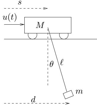
Figure 3.1.: Cart with pendulum
