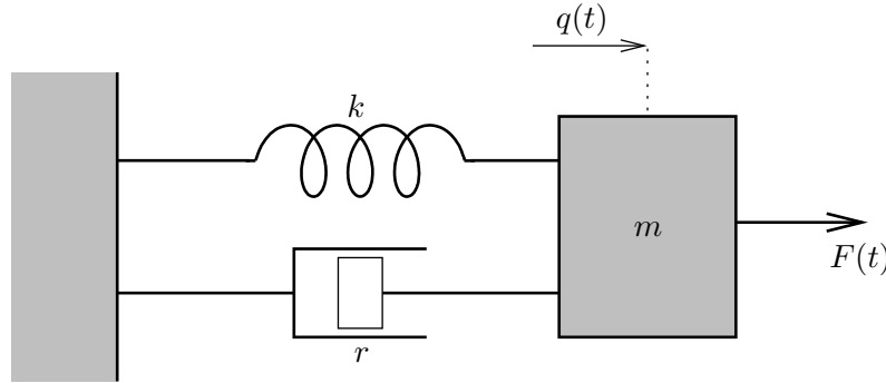
Figure 1.3.: Mass-spring-system
