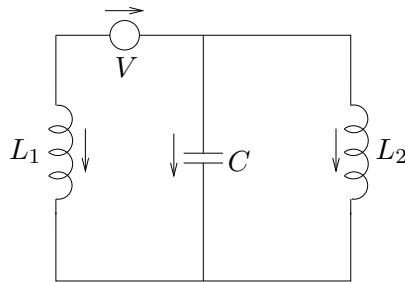
Figure 1.2.: Electrical network
