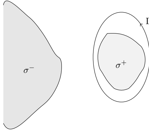
Figure 8.1.: spectral decomposition
